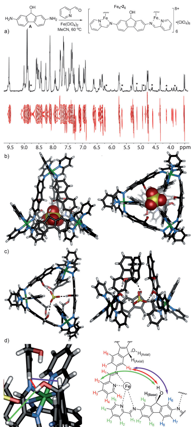
Figure 2. Characterization of [Fe 4 ·2 6 ] 8+ : a) 1 H NMR and 2D DOSY spectra of [(ClO 4 )·Fe 4 ·2 6 ] 7+ (CD 3 CN, 400 MHz, 298 K; Δ = 100 ms, δ = 2.6 μs, diffusion coefficient = 4.8 × 10 –10 m 2 s –1 ). * = minor peaks from other isomers. b) Crystal structure of the [(ClO 4 )·Fe 4 ·2 6 ] 7+ cage showing the presence of both \Delta - fac and \Delta - mer iron(II) centers and the bound perchlorate guest. c) Cropped views of the X-ray crystal structure of [(ClO 4 )·Fe 4 ·2 6 ] 7+ showing: hydrogen bonding between ligand and alcohols and the bound perchlorate and hydrogen bonds between different ligand alcohol groups. d) NOE contacts observed by NOESY analysis of the solution-phase structure (see SI for full assignment).
